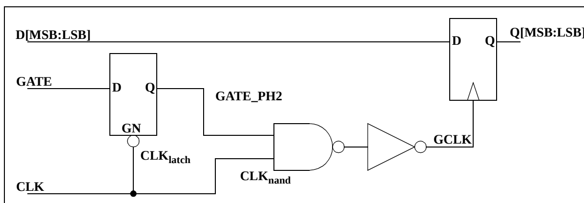
Figure 2. Gated Clocking Schematic
